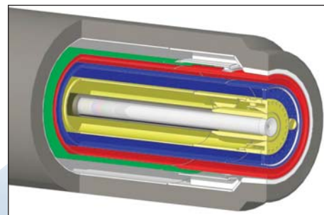
Nozzle closed
